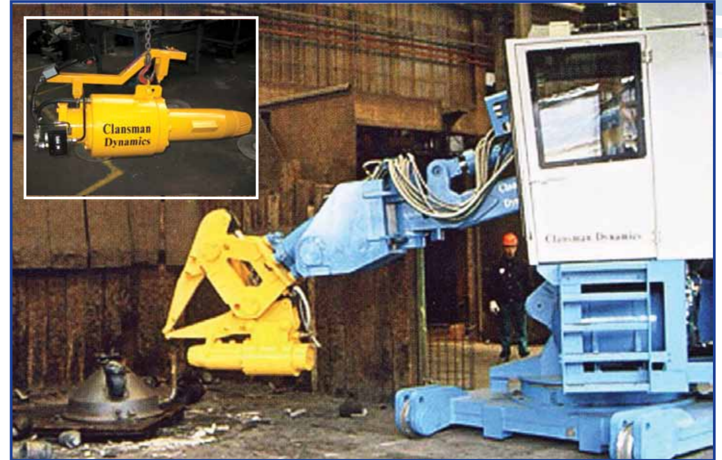
1. C 2010 Railbound manipulator with knock off hammer
