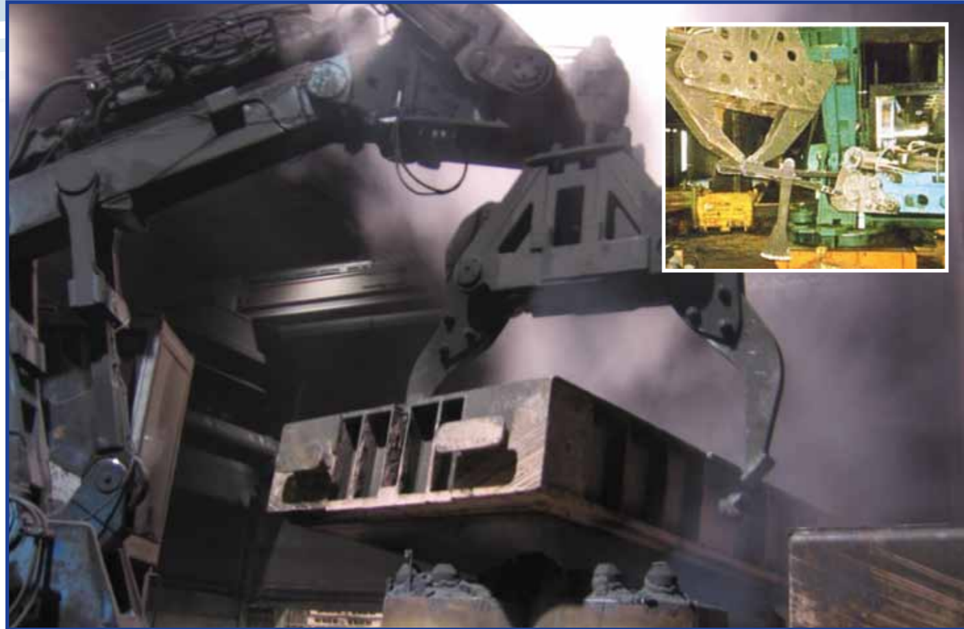
1. Manipulator C5010 (10 T mould boxes)
